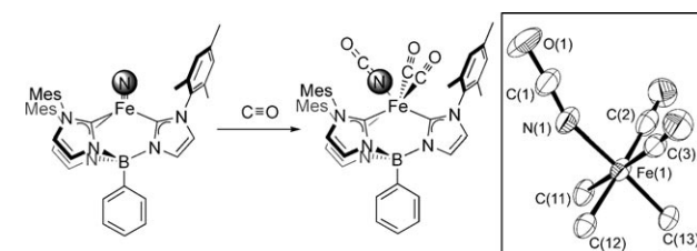
Figure 2. Synthesis of the isocyanate complex [L^{\text{Mes}}\text{Fe}(\text{NCO})(\text{CO})_2] . Inset: X-ray crystal structure. Ellipsoids set at 50% probability; hydrogen atoms and most of the tris(carbene)borate ligand omitted for clarity. Selected bond lengths [Å] and angles [°]: Fe1–N1 1.987(2), N1–C1 1.156(4), C1–O1 1.210(4); Fe1–N1–C1 159.8(3), N1–C1–O1 177.0(4).
