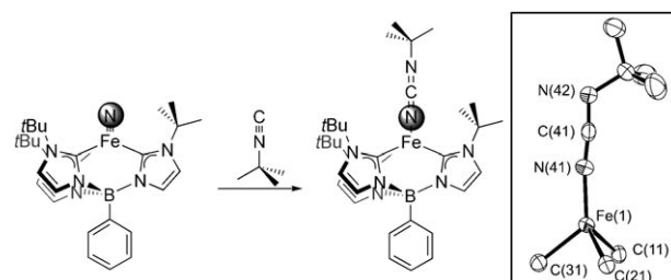
Figure 3. Synthesis of [L^{\text{tBu}}\text{Fe}=\text{N}=\text{C}=\text{NtBu}] . Inset: X-ray crystal structure. Ellipsoids set at 50% probability; hydrogen atoms and most of the tris(carbene)borate ligand omitted for clarity. Selected bond lengths [Å] and angles [°]: Fe1–N41 1.936(3), N41–C41 1.186(4), C41–N42 1.242(5); C41–N41–Fe1 169.8(3), N41–C41–N42 173.7(3).
